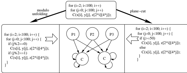
Figure 5: Modulo unfolding vs. Plane-cut
