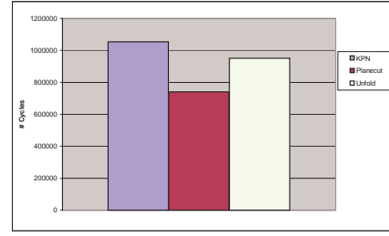
Figure 11: Diagonal dependencies: results on the Cell
