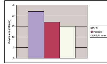
Figure 6: Results on the ESPAM platform
