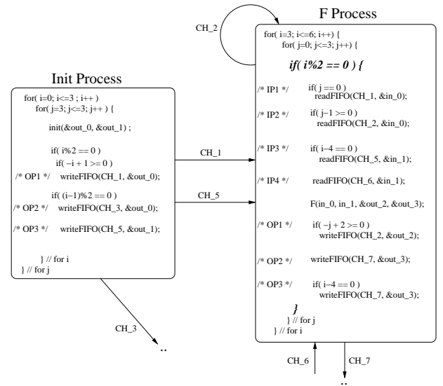
Figure 3: Structure of Unfolded Process F
