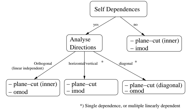
Figure 9: Decision Tree
