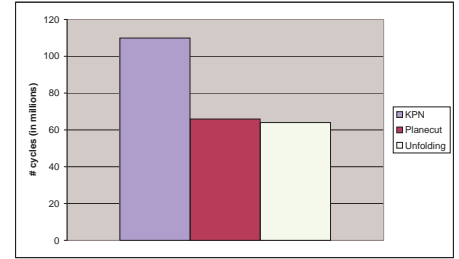
Figure 17: Results on ESPAM Platform
