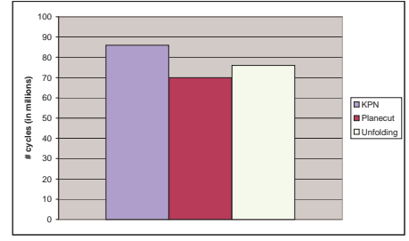
Figure 16: Results on the Cell
