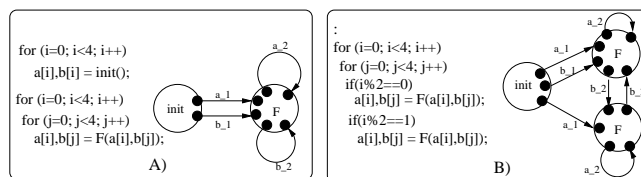
Figure 1: Kahn Process Network
